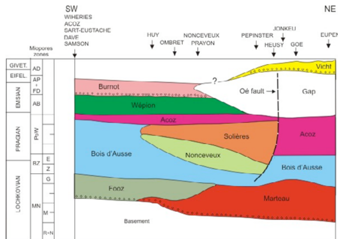
Fig. 9. — The Lower Devonian chart of Belgium.
